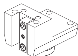
Face and O.D. cutting holder
