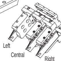
Protection cover 137-00272
