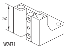
Face and O.D. cutting holder 20x20 mm
