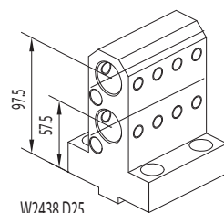
Double toolholder for boring bar Ø25 mm
