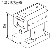
128-21803 Ø40 128-21806 Ø50
