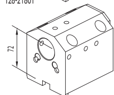
128-21802 Ø40 128-21805 Ø50
