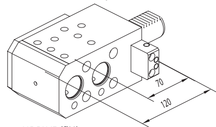
Double toolholder for boring bar
