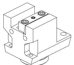
Face and I.D. cutting holder
